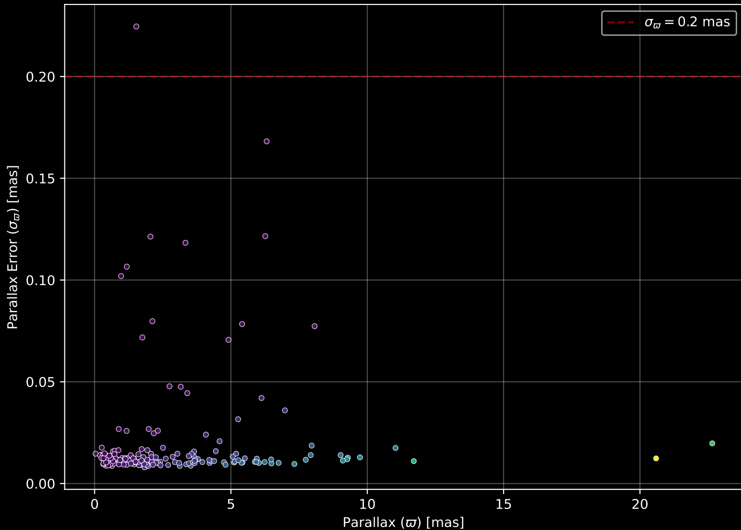
APOGEE DR17 Field: [265-31-O_TESS] Parallax Quality (n= 182)
