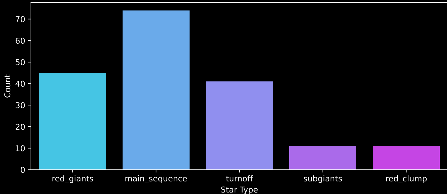
APOGEE DR17 Field: [265-31-O_TESS] Count plot of Star Type
