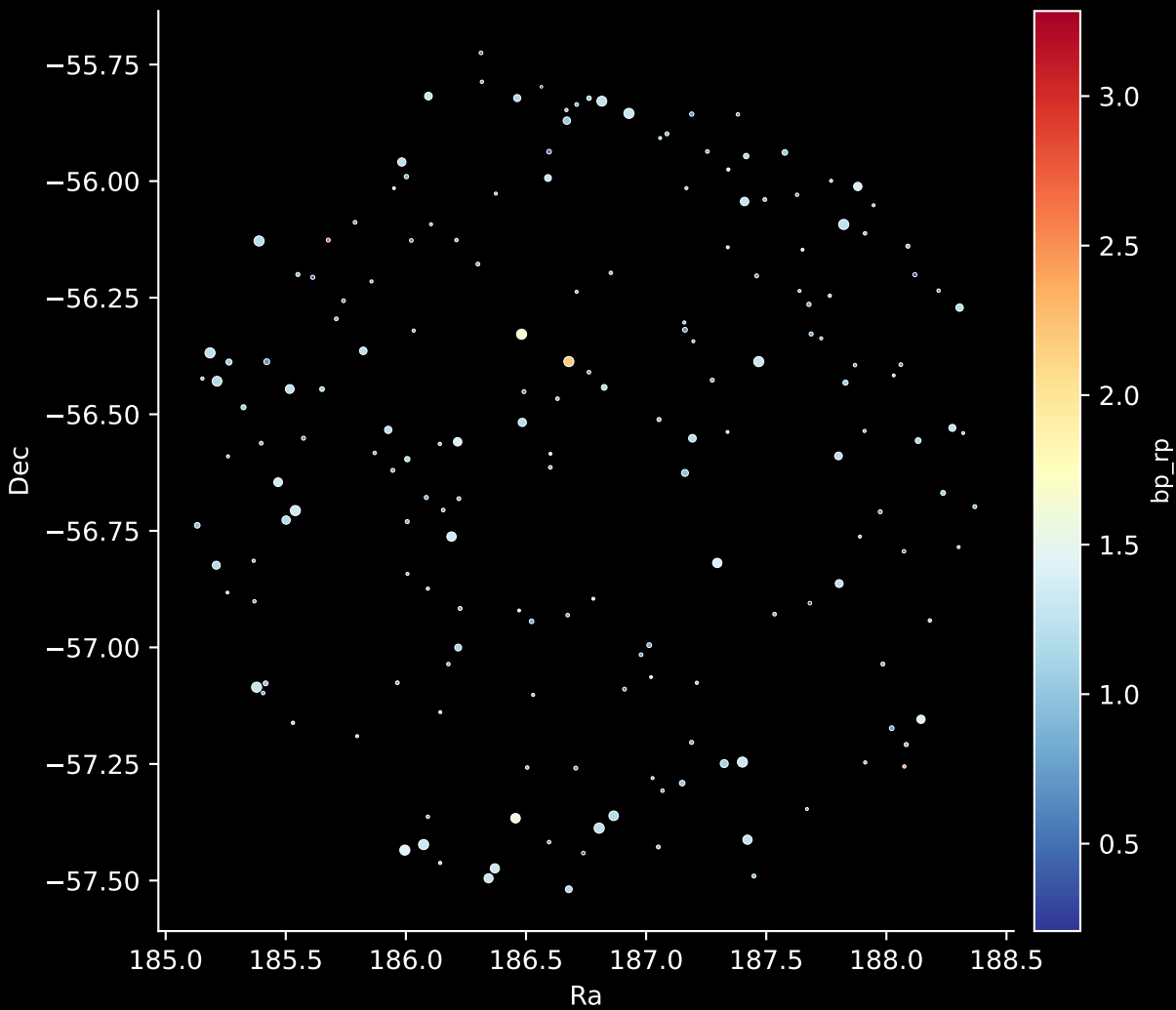
APOGEE DR17 Field: [265-31-O_TESS] Stars: 182
