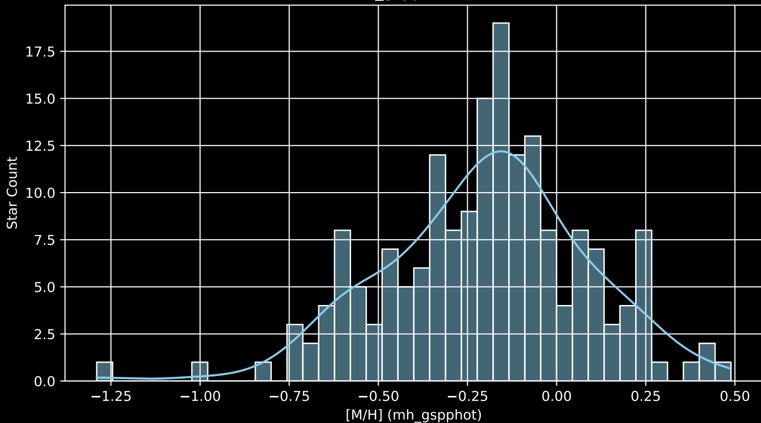
APOGEE DR17 Field: [265-31-O_TESS [M/H] (mh_gspphot) (n= 181)
