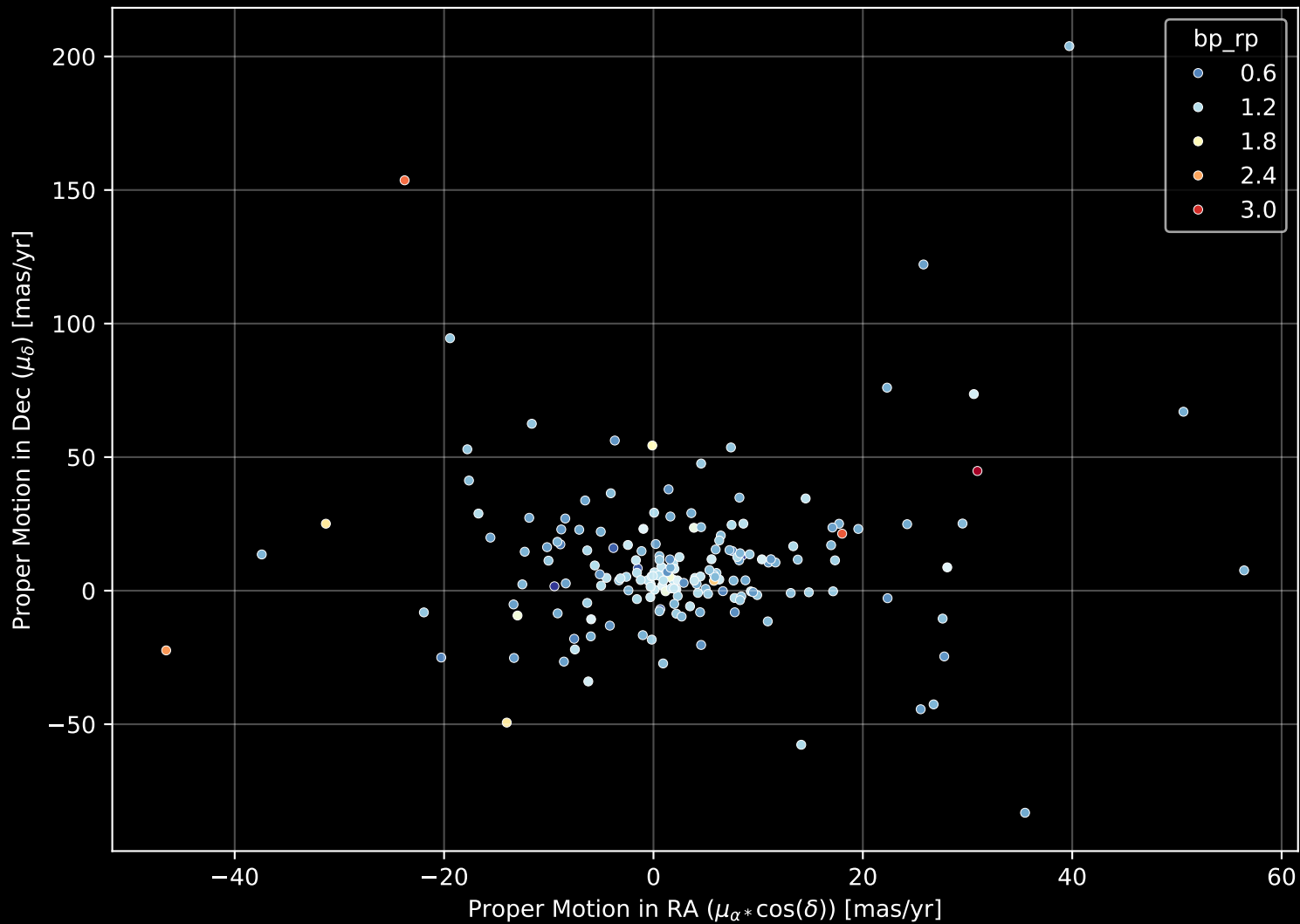
APOGEE DR17 Field: [265-31-O_TESS] Proper Motion Diagram (n= 182)
