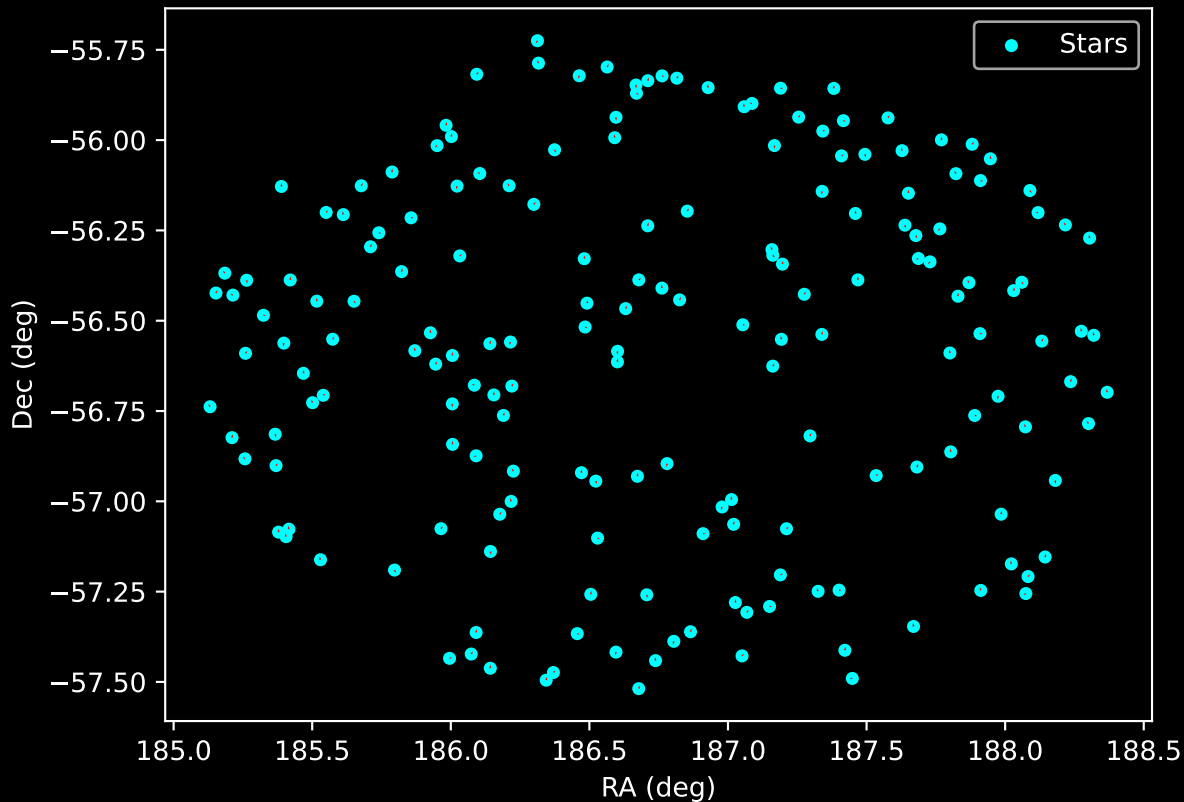
APOGEE DR17 Field: [265-31-O_TESS] Proper Motion Vectors for Gaia Star Field (n= 182)
