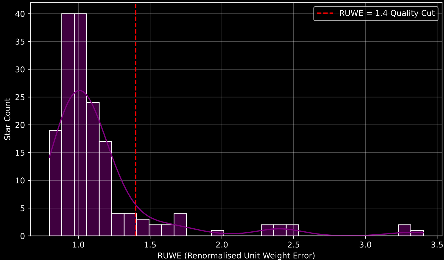
GAPOGEE DR17 Field [265-31-O_TESS] RUWE Distribution (n= 169)
